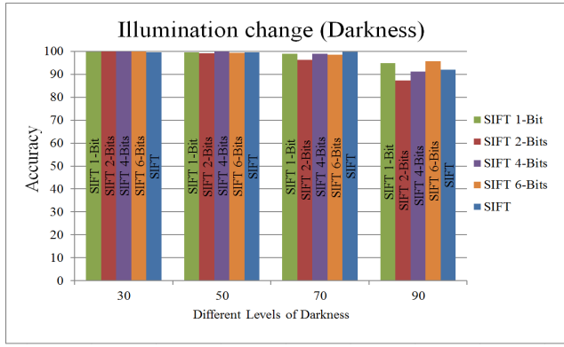
Figure 5: Matching performance of different reduction approaches compared with SIFT descriptor in the presence of darkness or reduction of light.
