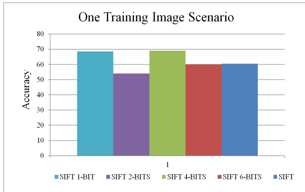
Figure 9: Matching performance of all different approaches in a scenario when there was only one train image in the database against each query image.
