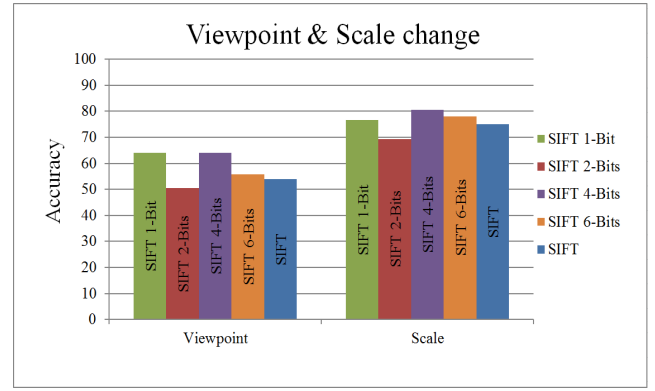
Figure 7: Matching performance of different reduction approaches in two different scenarios i.e. viewpoint and scale change.
