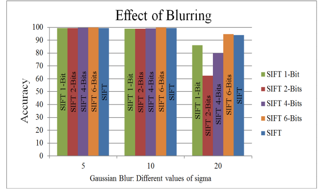
Figure 3: Matching performance against blurred images of three different sigmas (represented by x-axis) in Gaussian blur.
