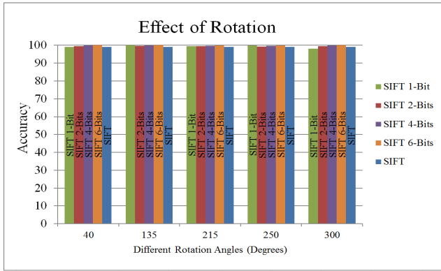
Figure 2: Matching performance in the presence of five different rotations angles applied to the train images.
