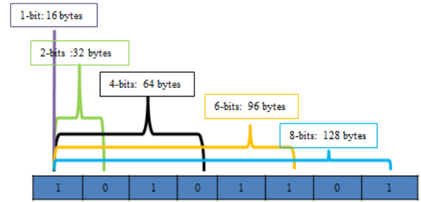
Figure 1: The suggested feature compression approach is illustrated. The total descriptor size is also displayed in bytes. Here x-bits means the number of bits kept from each dimension of the descriptor.
