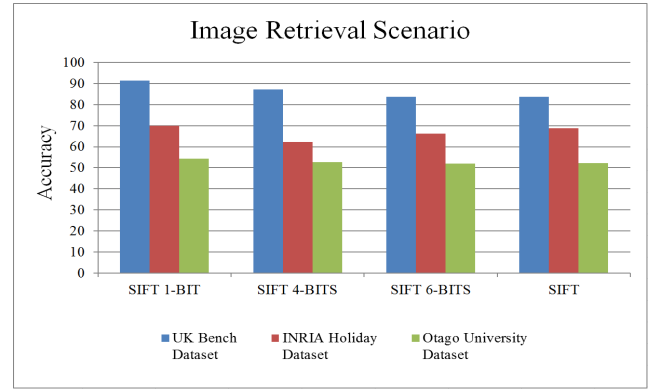
Figure 8: Matching performance of different reduction approaches in two different scenarios i.e. viewpoint and scale change.
