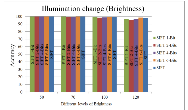
Figure 4: Matching performance of different reduction approaches compared with SIFT descriptor in the presence of brightness or addition of light.
