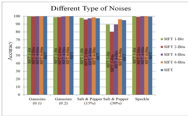
Figure 6: Matching performance of different reduction approaches compared with SIFT descriptor in the presence of different noise.
